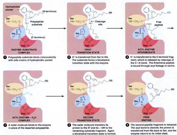
Figure 11.13 Catalysis of peptide bond hydrolysis by chymotrypsin
